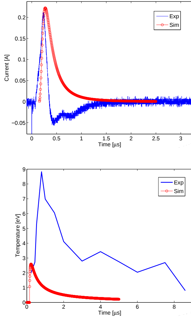
Figure 5.4.4: Up - Unbiased Langmuir probe signal detected at 14.5mm from the target compared with the simulated one. Down - Measured electron temperatures as function of the time in comparison with simulated one at the same position
