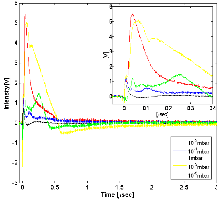
Figure 2.3.20: TOF signals vs. time at different background pressures for d_{LT} = 4.5\text{mm} .
