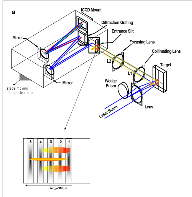
Figure 3.2.7: Schematic diagram of the optical spectroscopy system without the use of the Dove prism, showing the main optical components, used to image the plasma light onto the entrance slit.
