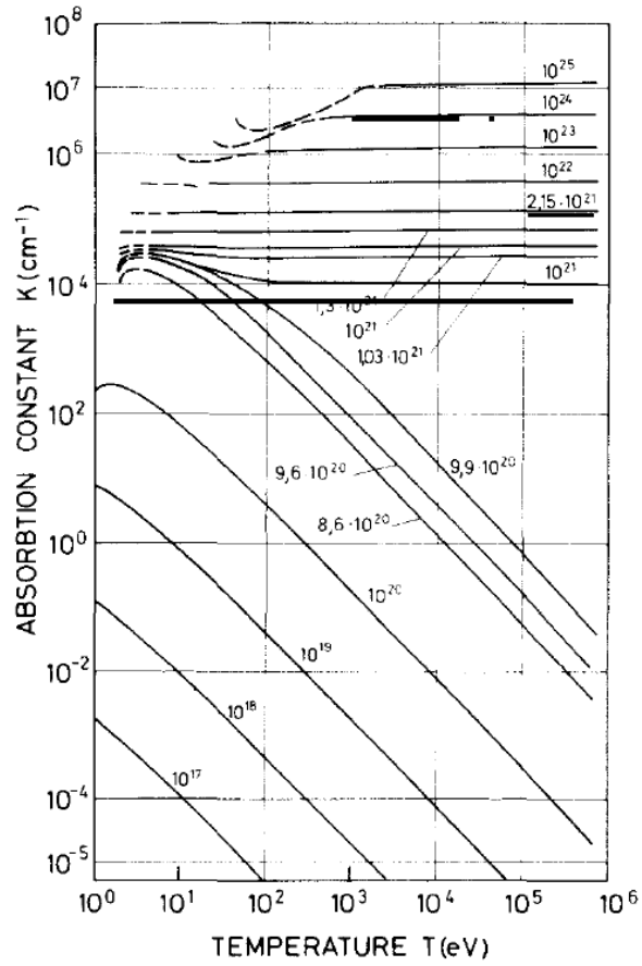
Figure 1.4.5: Optical absorption constant K vs plasma temperature T for a ND:Yag laser with wavelength equal to 1064\mu m for different electron densities taking into account the Spitzer collisions [22] .
