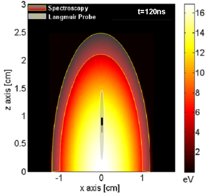
Figure 5.4.3: 2D simulation of the Al plume in terms of plasma temperature at a fixed time expansion; the area in which the probe is located indicates the experimental region where LP measurements were made; the area of the coronal plasma was instead investigated experimentally by time resolved spectroscopy.
