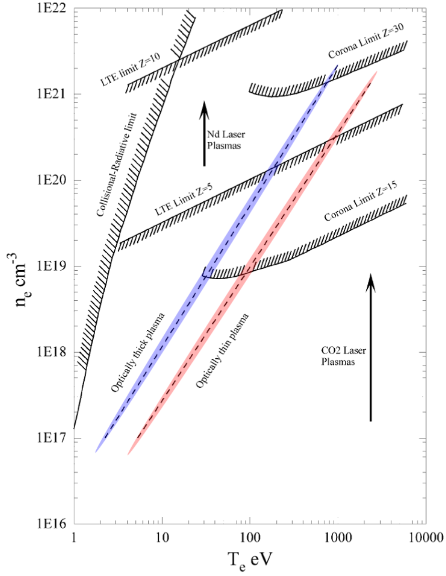
Figure 1.5.1: Electron density and Electron temperature ranges for applicability of LTE, CE, and CR models [23].
