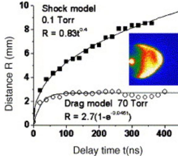
Figure 1.9.1: Rt plot for the expanding aluminum plasma plume front in ambient nitrogen atmosphere at 0.1 and 70 Torr. Inset shows the formation of shock wave at 0.1 Torr [40].
