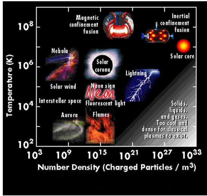
Figure 1: Classification of Plasmas vs temperature and Density (DOE Fusion Lab-NASA).
