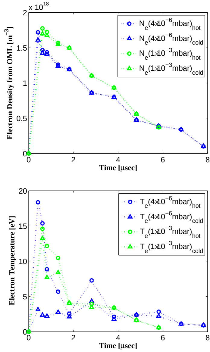
Figure 2.3.22: Electron Densities and Electron Temperatures vs time @ 4 \cdot 10^{-6} \text{ mb} and @ 1 \cdot 10^{-3} \text{ mb} @ 4.5 \text{ mm} from the target.
