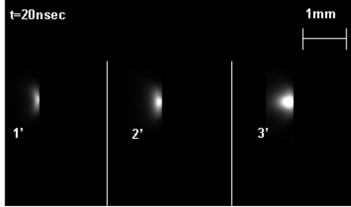
Figure 2.3.3: CCD Images obtained with three consecutive shots, obtained at 100ns.
