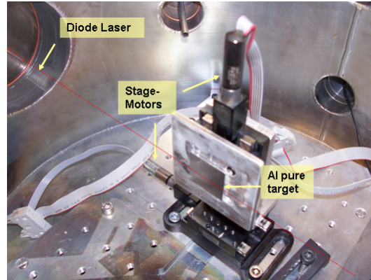
Figure 3.2.2: Motorized target holder for the Al target, aligned by means of a red diode Laser.
