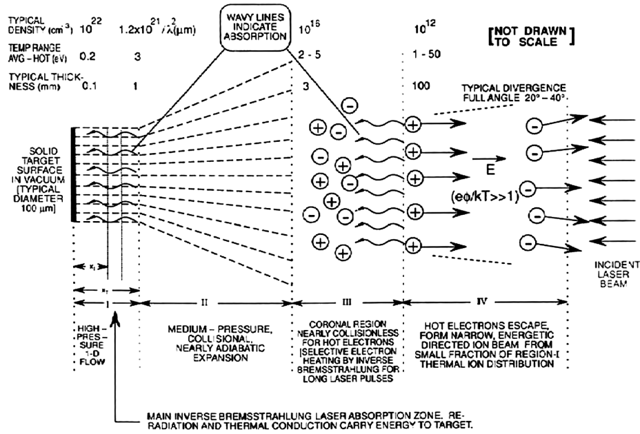
Figure 1.8.1: General expansion dynamics scheme of a laser generated plasmas, for spot sizes on the order of 100 \mu m and laser energies on the order of 5 – 10J/cm 2 (from Laser Ionization Mass Analysis, C. R. Phipps, R. W. Dreyfus, 1993 J. Wiley & Sons).
