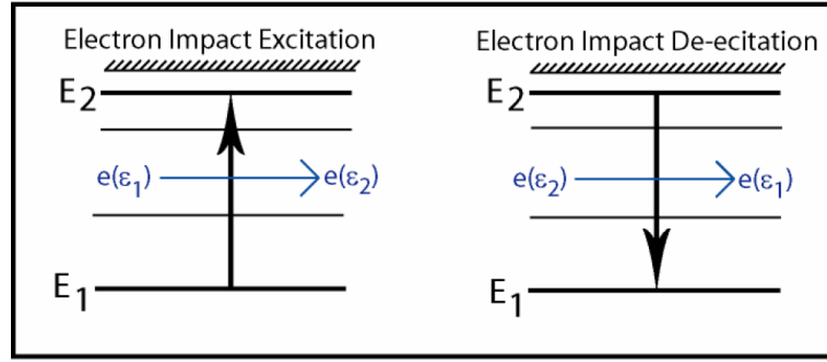
Figure 1.4.3: Schematic diagram of the electron impact excitation (left) and electron impact de-excitation (right) atomic processes which occur in laser produced plasmas.
