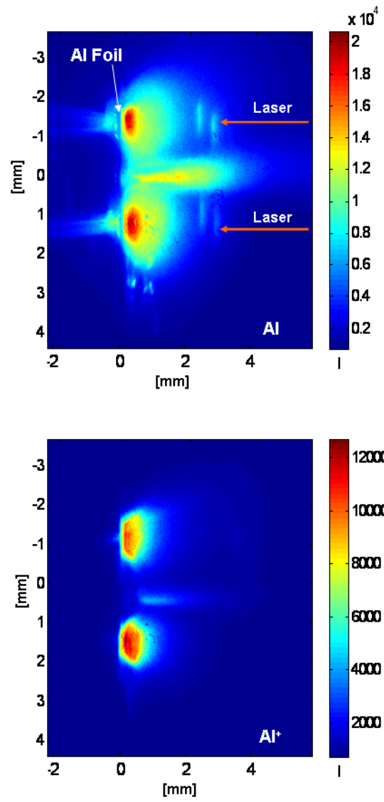
Figure 4.3.1: Time integrated images of colliding plasmas: broadband imaging (top), ion imaging (down) .
