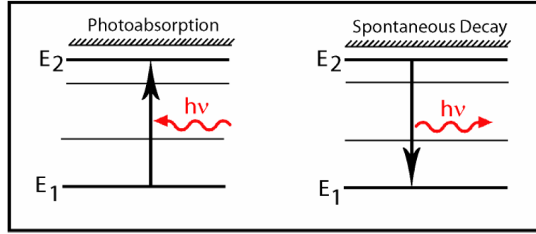
Figure 1.4.6: Schematic illustration of the photoabsorption (left) and spontaneous decay (right) processes. E_1 and E_2 are lower and upper electron energy states of the atom/ion respectively.
