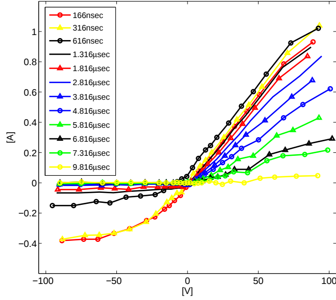
Figure 2.3.17: I-V curves obtained when the probe was located orthogonally to the plume expansion direction at 15mm from the target.
