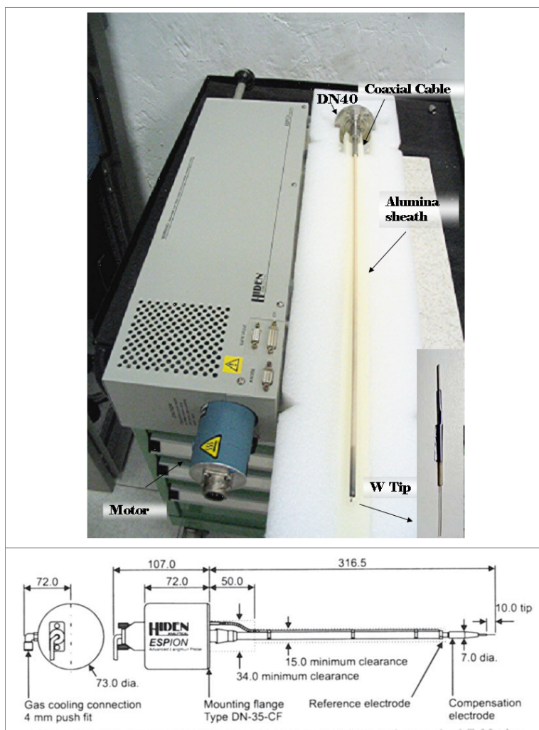
Figure 2.2.4: Langmuir Probe and W Tip (up), technical draft of the LP (down).
