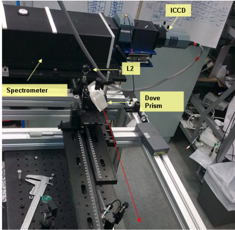
Figure 3.2.9: Picture of the optical spectroscopy set-up, when the dove prism was located between L_1 and L_2 ; the red arrow indicates the direction of the incoming plasma radiation.
