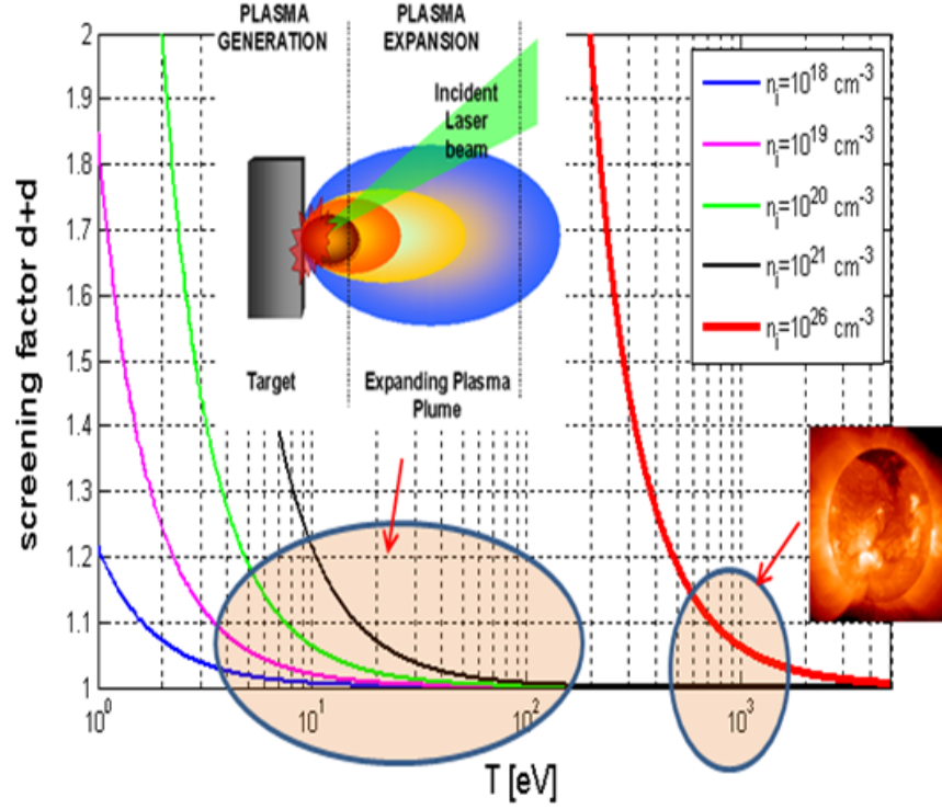
Figure 2: Screening factor for D+D reaction as a function of electron temperature and density. On the right plane, highlighted the typical solar values. In the central region an highlighted the temperature and density obtained from the plasma induced by laser ablation [2].
