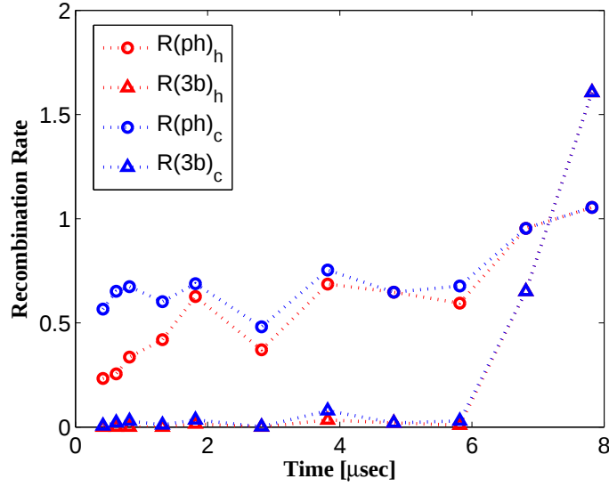
Figure 2.3.11: Recombination Rate vs time for d_{LT} = 4.5mm .
