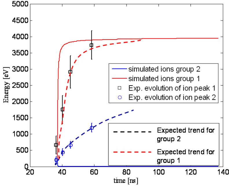
Figure 2.3.15: Comparison between the simulated ion and electron bunches energies and the experimental energies obtained from the TOF signals reported in section 2.3.1.
