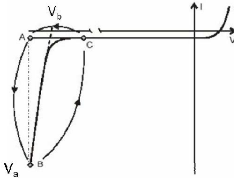
Figure 1-4: I-V characteristic of SPAD device operating in a Geiger mode.
