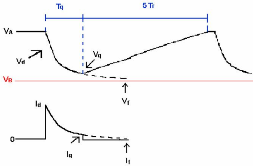
Figure 1-5: Voltage oscillation and current production during photon detection of SPAD device with PQC.
