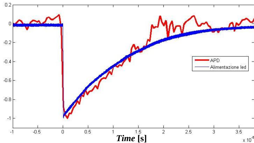
Figure 3-18: APD measurement of high intensity modulated light source.
