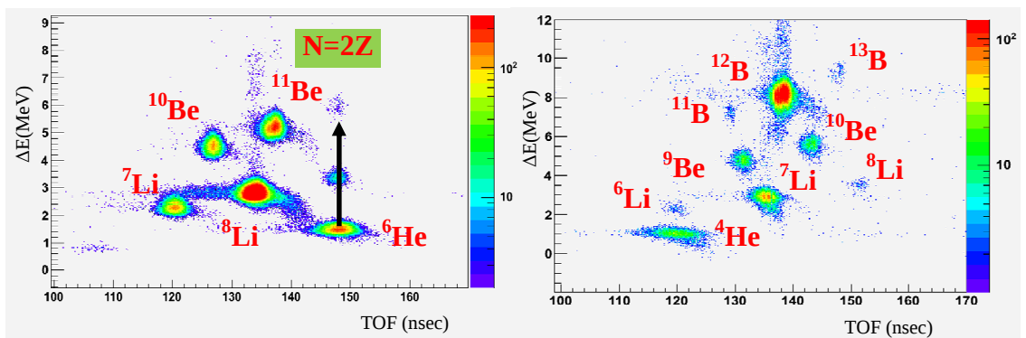
Figure 2.7 ^{13}\text{C} primary beam at 55 MeV/u and ^9\text{Be} production target 1,5 mm. Energy loss in the DSSD against the time of flight between the silicon detector and the MCP. The picture corresponds to the magnetic field configuration to optimize the ^{11}\text{Be} transport. The lower one corresponds to the optimization of ^{12}\text{B} . The black line shows element with the same time of flight.
