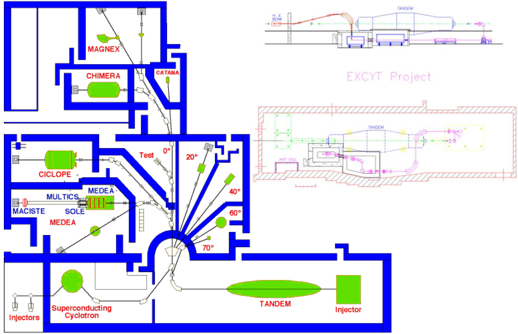
Figure 2.2 Layout of the LNS-INFN laboratory and EXCYT facility [LNSW].
