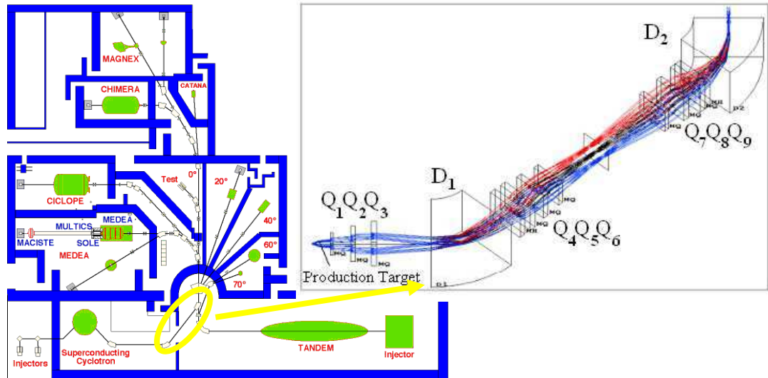
Figure 2.6 Layout of the LNS and the Fragment Recoil Separator used to select exotic beams [LNSW].
