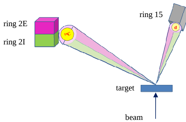
Figure 4.11 Schematic view of a typical coincidence between two telescopes along the polar angle.
