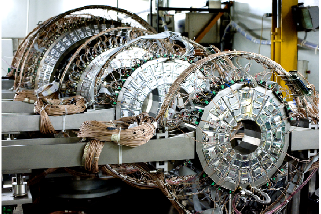
Figure 3.2 Recent photo of the CHIMERA multidetector with sphere and five rings. The other four rings of the forward part have been transferred at GSI.
