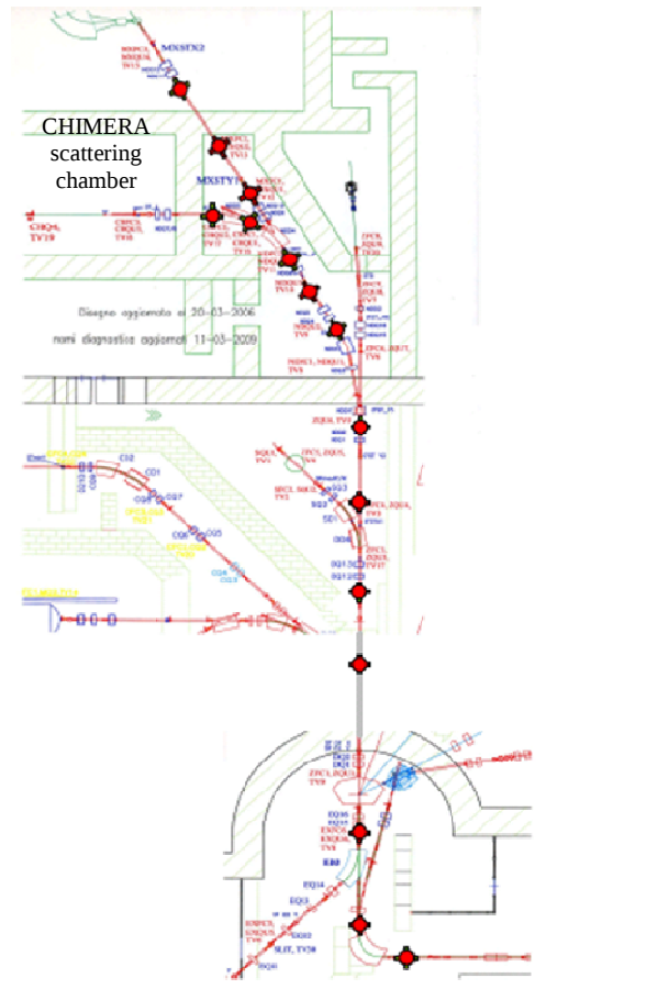
Figure 2.10 Schematic view of the beam line. The diagnostic points are marked with the red circles [COS09].
