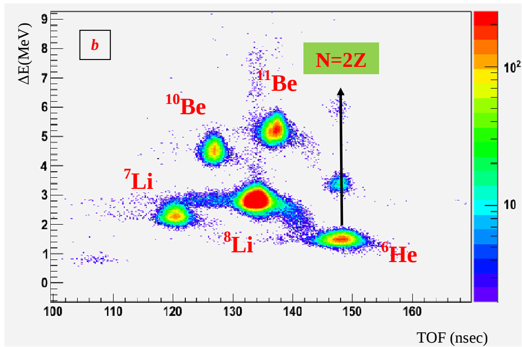
Figure 4.3 ^{13}\text{C} primary beam impinging on ^9\text{Be} production target. Magnetic field setting optimized to the transport ^{11}\text{Be} . (a) TOF - \Delta E LISE++ code simulation. (b) Experimental data TOF - \Delta E scatter plot.
