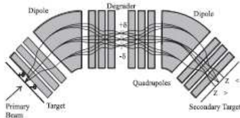
Figure 2.5 Schematic representation of the ion-optics used in a momentum-loss achromat to separate projectile fragments [MOR04].
