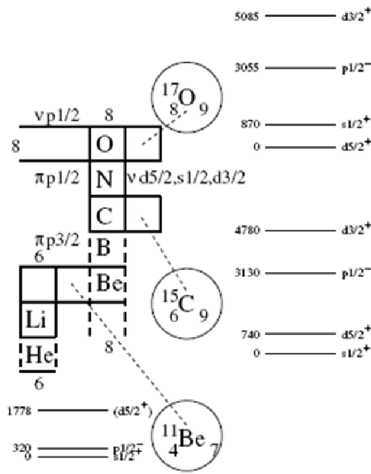
Figure 1.3 Examples of shell inversion [GRA04].
