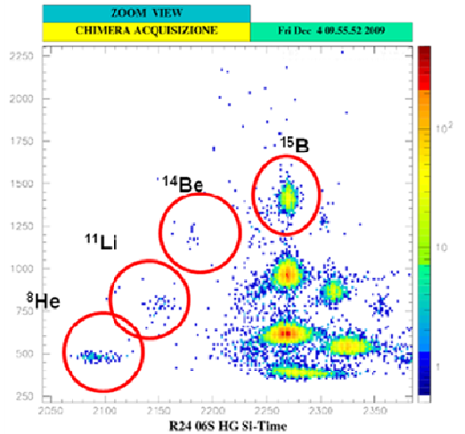
Figure 2.9 Scatter plot \Delta E -TOF. ^{18}\text{O} primary beam at 55 MeV/A impinging on a ^9\text{Be} production target [AGO09].
