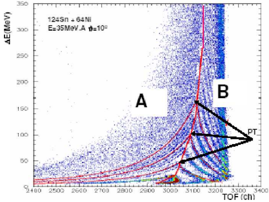
Figure 3.9 Reaction ^{124}\text{Sn} + ^{64}\text{Ni} at 35 MeV/u. TOF scatter plot. Time of flight against the energy measured by the silicon detector. The A side shows particles stopped in the Silicon detector, the B side particles punching through.
