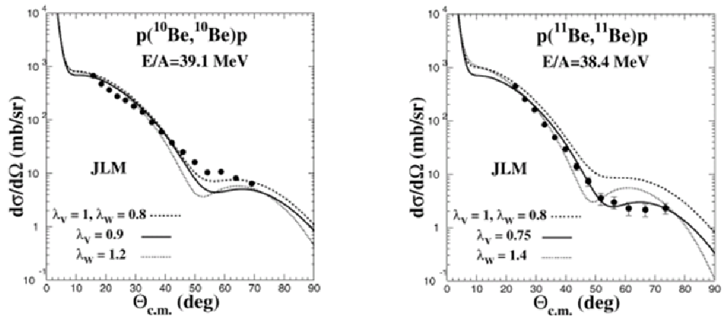
Figure 1.6 On the left side the cross sections for the ^{10}\text{Be} + p elastic scattering at 39.1 MeV/u compared to calculations using the JLM potential and the “Sagawa” density. The full circles correspond to the data. The dashed line corresponds to the standard JLM calculation for light nuclei. Full line (dotted line) corresponds to calculations in which the real part (imaginary) was renormalized. The potential is written: U_{\text{JLM}} = \lambda_V V + i\lambda_W W , with \lambda_V , \lambda_W the normalization factors of the real V and imaginary W parts of the potential. On the right side ^{11}\text{Be} + p elastic scattering at 38.4 MeV/u [LAP08].
