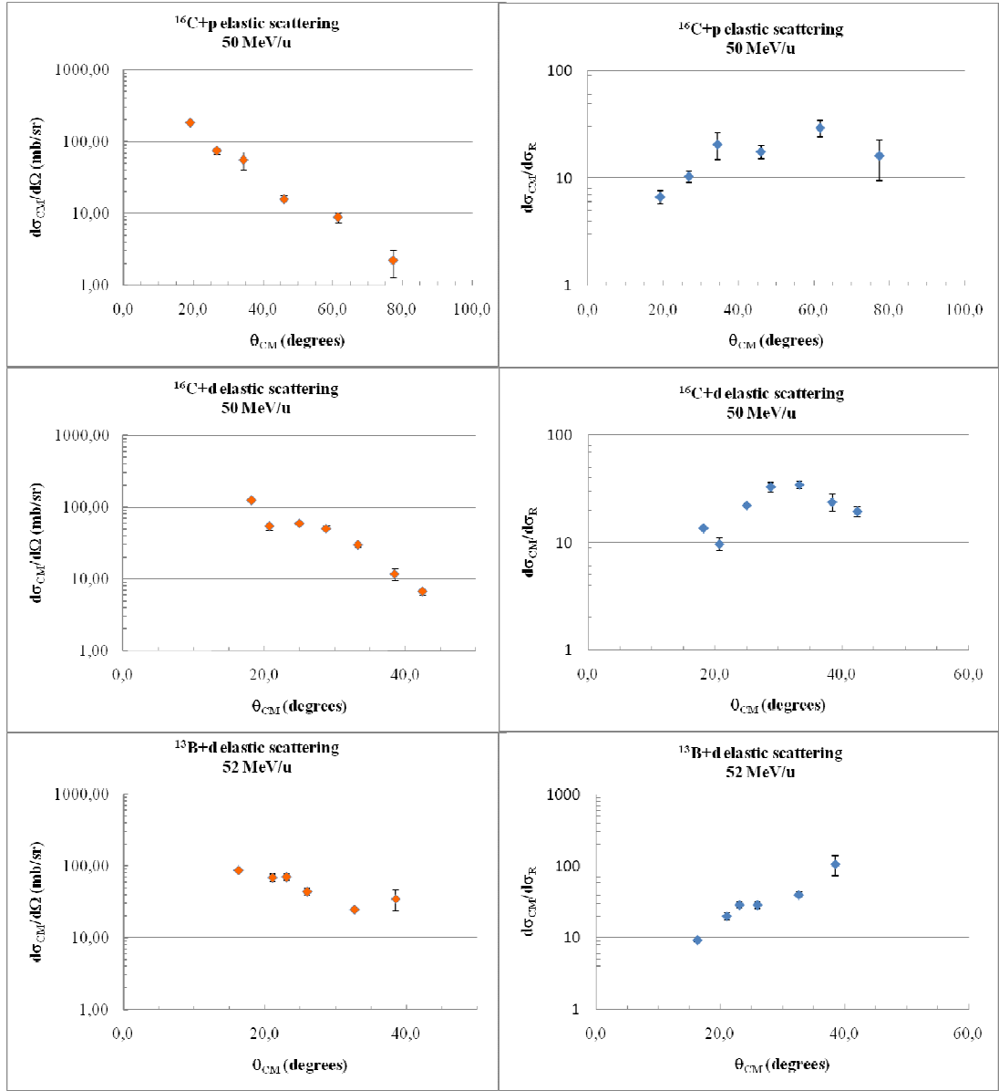
Figure 4.14 Elastic scattering angular distribution for colliding systems. On the left side the measured cross section. On the right side the ratio to the Rutherford cross section.
