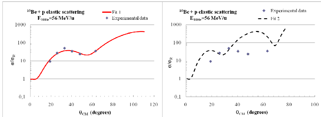
Figure 5.4 ^{10}\text{Be}+p elastic scattering. The panels show two data fits corresponding to the parameters summarized in Table 5.3.
