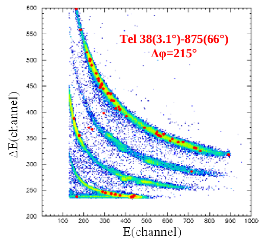
Figure 4.8 Selecting ^{12}\text{B} beam, the red points correspond to the particles detected in the telescope at 3.1^\circ in coincidence with the telescope at 66^\circ . The missing elastic events are due to \Delta\phi=215^\circ .
