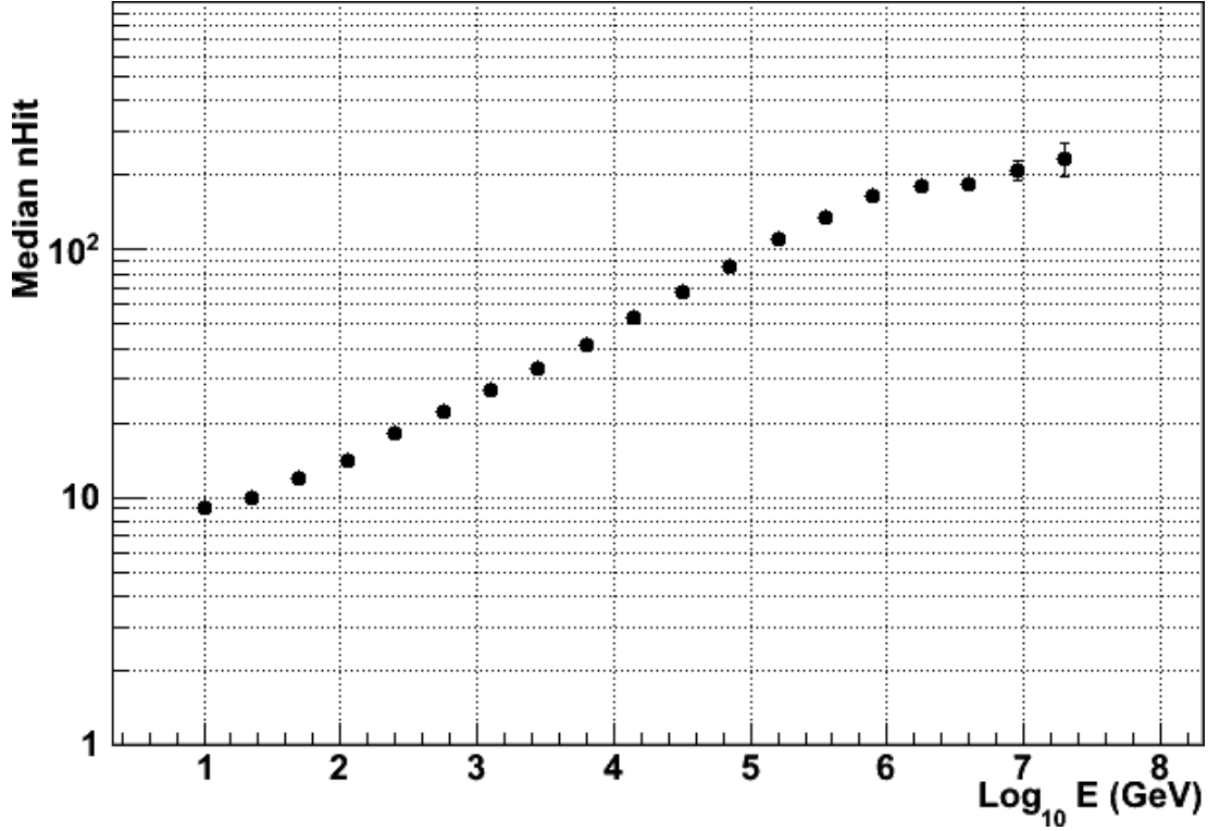
Figure 6.1: nHit Spectrum - The median of the number of hits used in reconstruction procedure after background hits cleanse (nHit) versus the generated neutrino energy E_\nu
