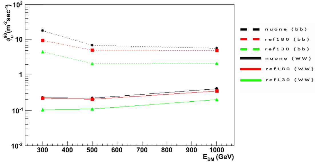
Figure 6.22: Sensitivity - Expected sensitivity for the three layouts (in different coloured lines) and all the considered models and channels (hard channel in solid lines, soft channel in dotted lines) after 5 years of full detector data taking
