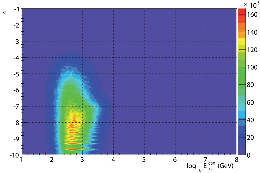
Figure 6.7: Muon \Lambda Distribution - \Lambda distribution of upgoing reconstructed muon events in the ref130 detector. The distribution is clearly peaked at \Lambda smaller than -7.
