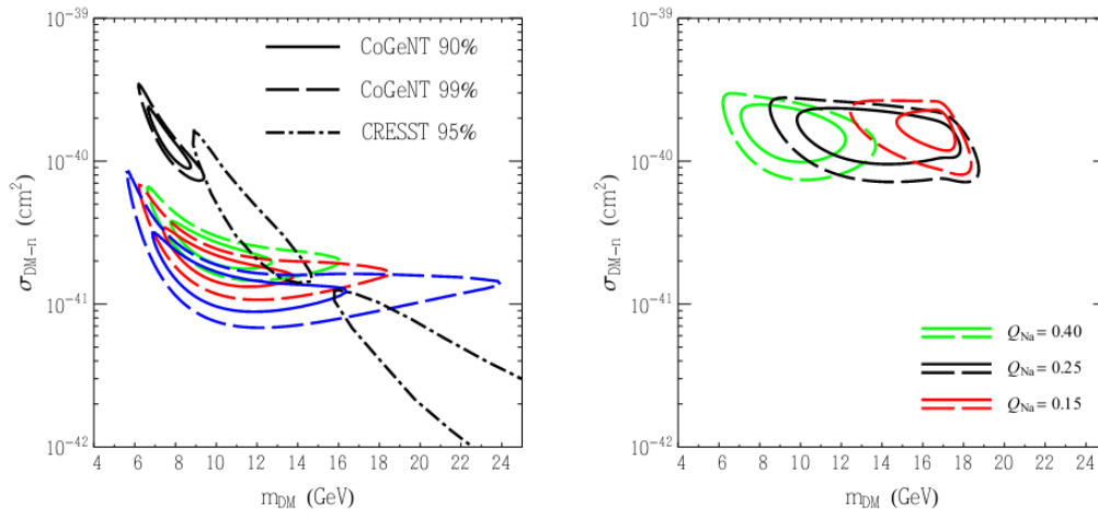
Figure 2.6: DAMA-CRESST-CoGeNT - Left - The 90% (solid) and 99% (dashed) confidence level contours for the spectrum of events observed by CoGeNT, The CRESST contours (dot-dashed) denote the 95% confidence level regions. A dark matter particle with a mass of approximately 10-20 GeV and an elastic scattering cross section with nucleons of approximately 10^{-41} \text{ cm}^2 can account for the excess events reported by each of these experiments. Right - The 90% (solid) and 99% (dashed) confidence level contours for the spectrum of the amplitude of the annual modulation observed by DAMA/LIBRA, assuming a simple Maxwellian velocity distribution with v_0 = 220 km/s and v_{\text{esc}} = 544 km/s. Taken from (23)
