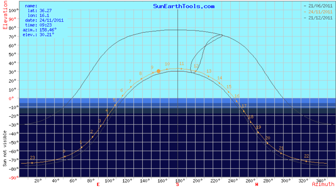
Figure 6.9: Sun Path - The expected path of the Sun in the detector frame, reflecting its apparent motion, taken from www.sunearthtools.com
