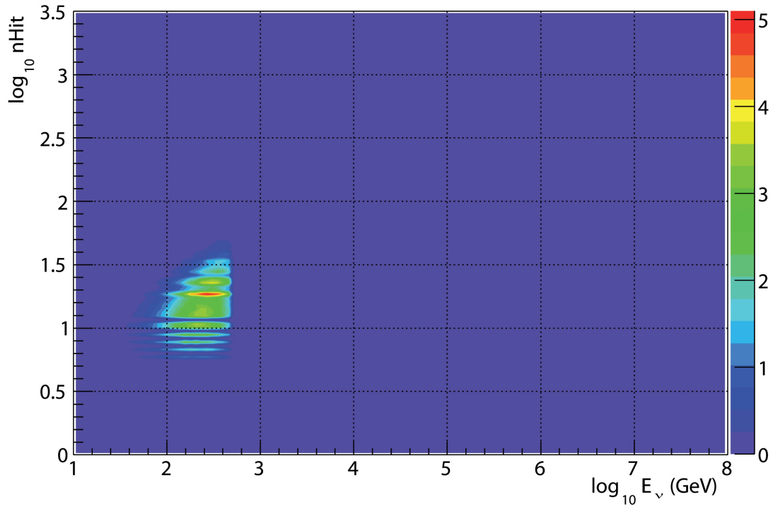
Figure 6.4: Sun nHit - The number of hits per reconstructed signal neutrino event versus the generated energy, at reconstruction level for the ref130 layout. The signal refers to 500GeV DM particle annihilating in the Sun through hard channel.
