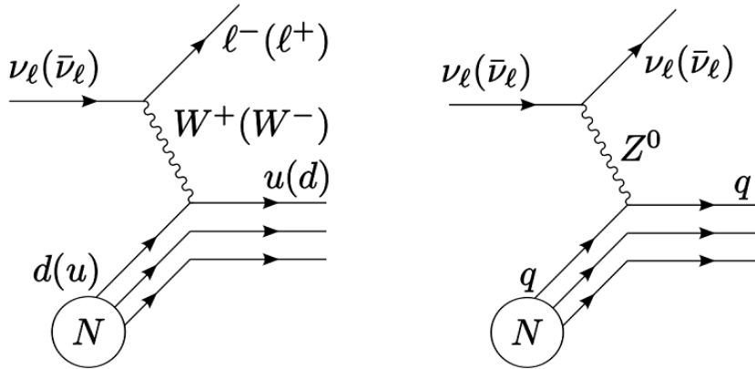
Figure 4.1: Neutrino Interactions - Left: Charged Current interaction - Right: Neutral Current Interaction
