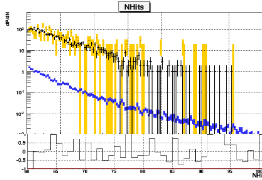
Figure 6.13: Upper panel: Distribution of the number of hits for the sample with the first level cuts applied (see text) for data (black), atmospheric muons (yellow) and atmospheric neutrinos (blue). Lower panel: (\text{Data} - \text{MC})/\text{MC} ratio.
