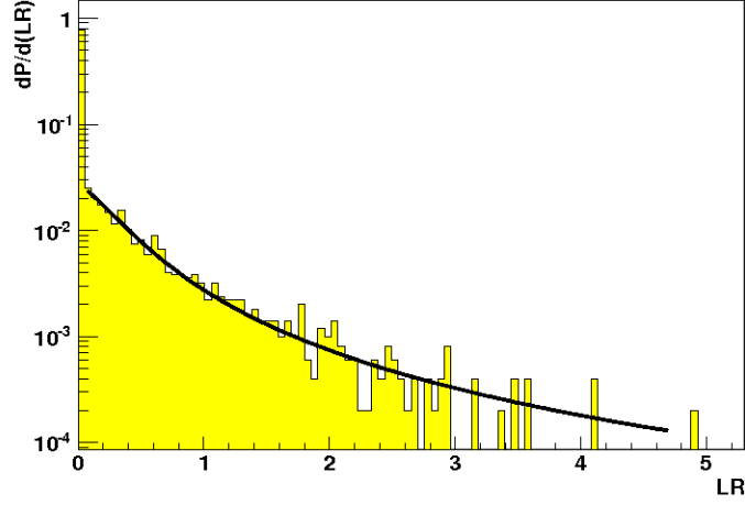
Figure 6.3: \frac{dP}{dLR} probability for the only-background case for 2 years of data taking. The black line is the fit with a \chi^2_{2n_{\text{dof}}} distribution. The geometry has a distance between the DU of 180 m.
