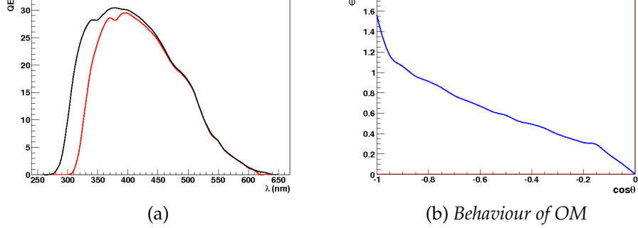
Figure 3.5: Left: The QE (unit %) (black line) a function of the wavelength of the photon and QE that includes the optical transmittance of the glass sphere and the gel (red line). Right: The angular acceptance of the PMT \epsilon including the effect of the optical ring ( \theta is the angle between the incident photon and the axis of the PMT, where \cos\theta = -1 corresponds to a head-on angle of incidence).
