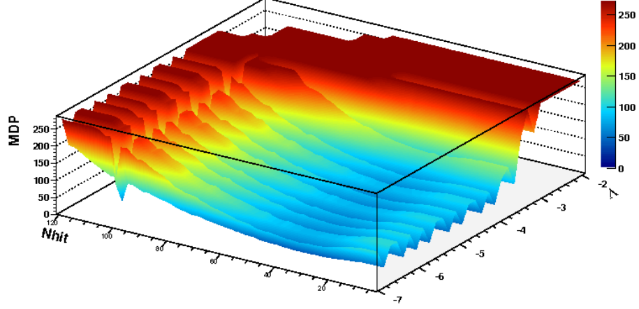
Figure 5.6: MDP minima in 2-dimensions with the detector geometry of reference [95] for one year of data taking in function of \Lambda and N_{\text{hits}} .
