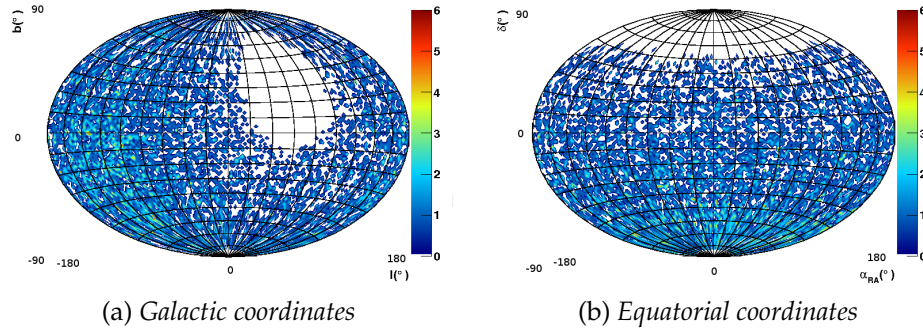
Figure 5.7: Monte Carlo sample for the background atmospheric neutrinos (in two different coordinates systems) with a geometry of 154 towers for one year of data taking. Only up-going events \theta_{rec} \leq 90^\circ are shown.
