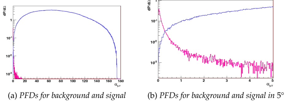
Figure 6.8: PDFs for background (blue) and signal (pink) for \delta = -60^\circ for a geometry with a distance of DU = 180m. Histograms are normalized to the number of events attended for 1 year of data taking.
