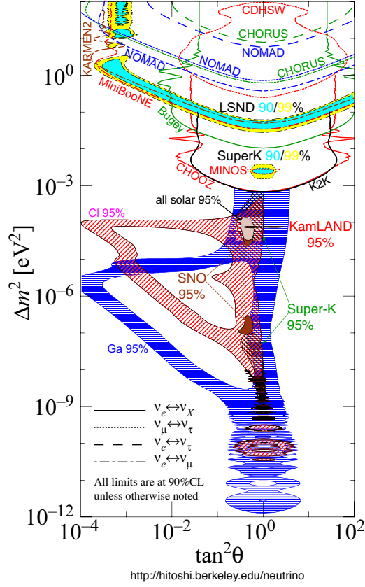
Figure 2.1: The regions of squared-mass splitting and mixing angle favoured or excluded by various experiments. References to the data used in the figure can be found at http://hitoshi.berkeley.edu/neutrino .
