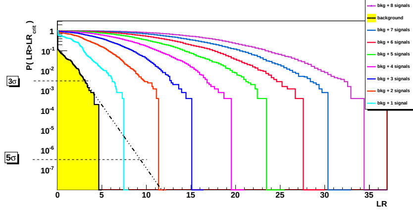
Figure 6.6: Integrated LR for the only-background case (yellow area) and for background + signal events (colored lines). Fitting the yellow histogram can be deduced the critical value at 5\sigma , LR_{5\sigma} , and then the probability value for the case signal+background. Geometry 1.
